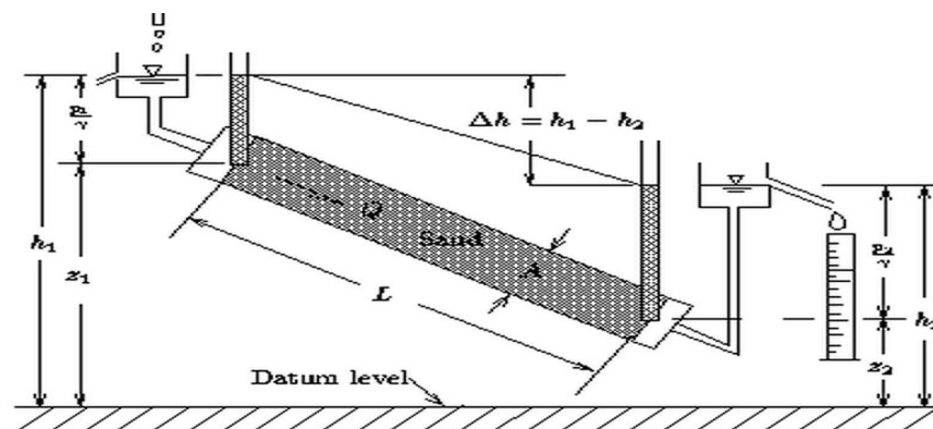
Figure 1. The flow through the sand-column to demonstrate the law of Darcy [9]
